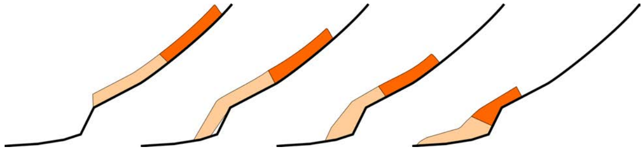
Figure 72. Schematic model of the successive stages of "Jumping" rock avalanche formation
