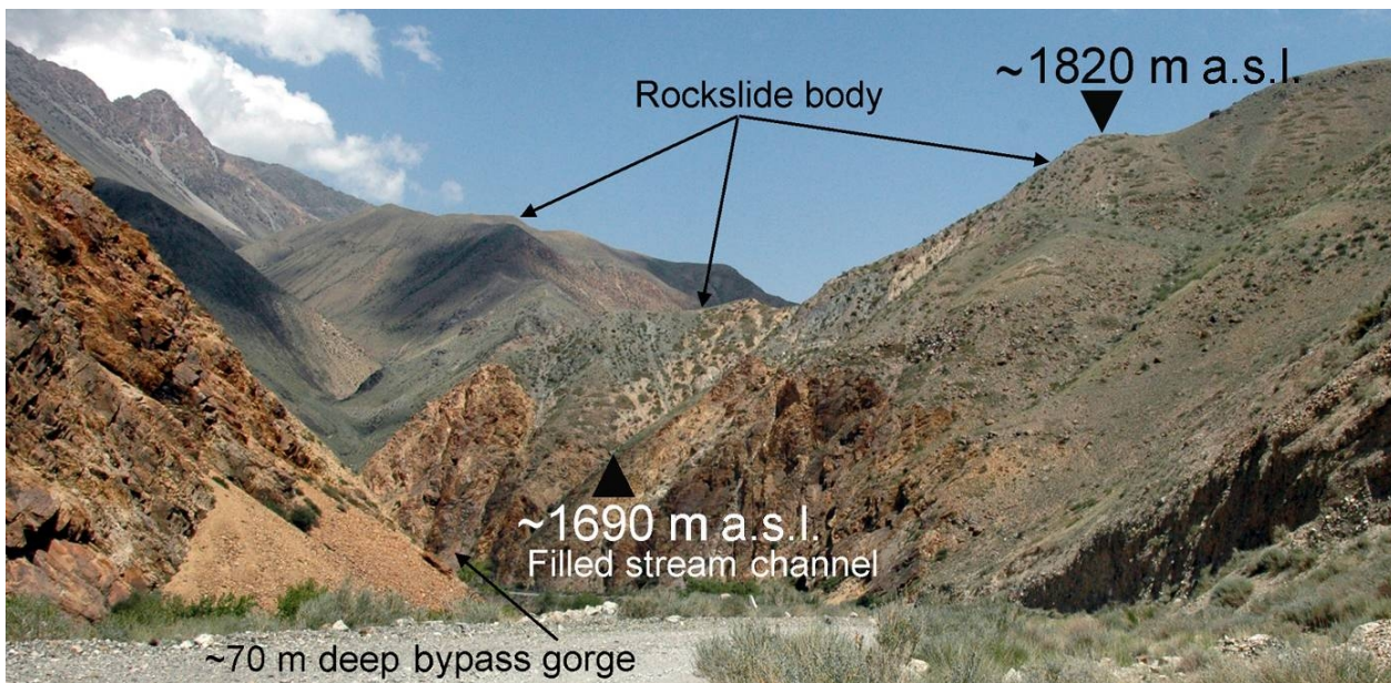
Figure 128. New gorge of the Kokomeren River that was incised after the blockage
