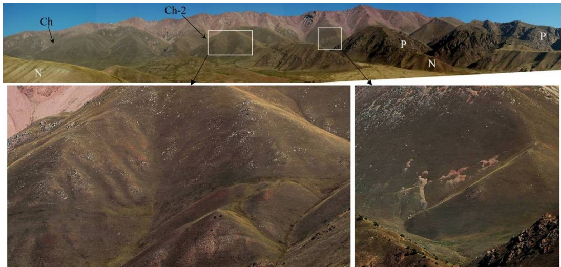
Figure 10. Surface ruptures along the North-Kyzyl-Oi fault zone.
